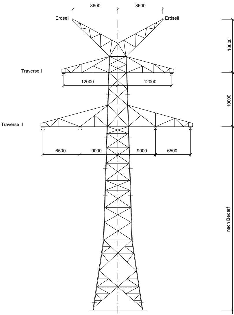
Winkelabspannmast WA140; D-2-D-2018.2 Mast-Nr.: 10, 23, 25, 32, 36, 37, 53, 54, 56, 58, 60, 61, 62, 64, 65, 73
