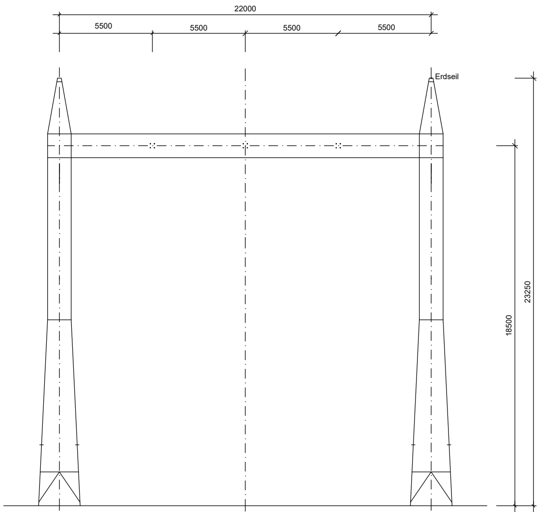
380-kV-Portal SE-380-KA-18.50-22.00-W4E2-2023.0 WOLK_C02, WOLK_C12
