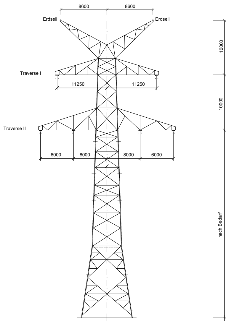
Winkelabspannmast WA160; D-2-D-2018.3 Mast-Nr.: 17, 19, 34, 48, 70
