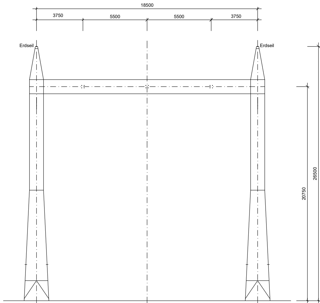
380-kV-Portal SM-380-UW-20.75-18.50-W2E3-2017.0 RAIW_C26; RAIW_C28
