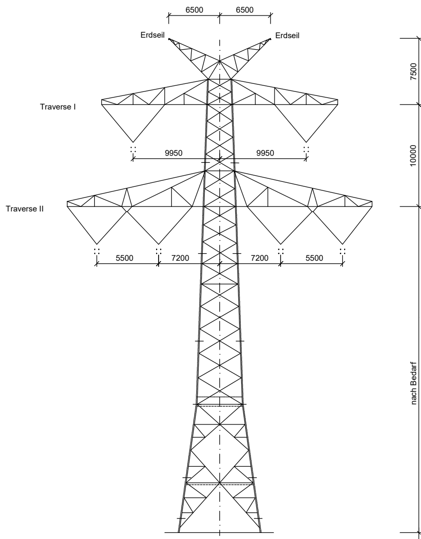
Tragmast T1; D-2-D-2018.3 Mast-Nr.: 2, 4, 5, 7, 9, 18, 26, 28, 41, 46, 47, 50, 71
