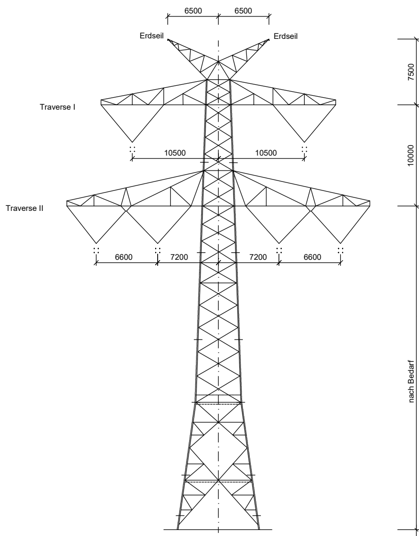
Tragmast T2; D-2-D-2018.2 Mast-Nr.: 12, 14, 15, 52, 59, 63
