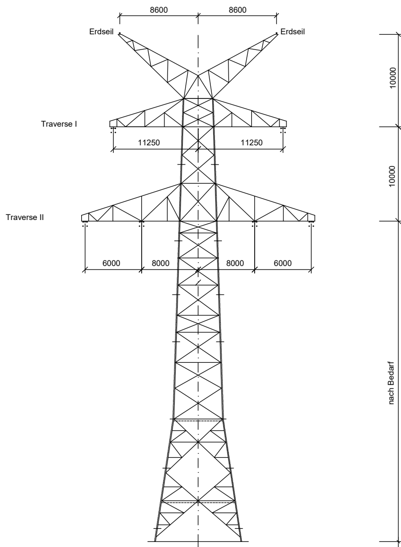
Winkelabspannmast WA160; D-2-D-2018.2 Mast-Nr.: 21, 66, 68, 77, 80, 82, 86, 88, 90
