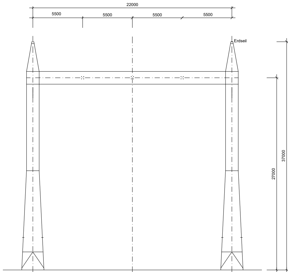
380-kV-Portal SE-380-KA-27.00-22.00-W4E2-2018.1 KATW_C02, KATW_C12
