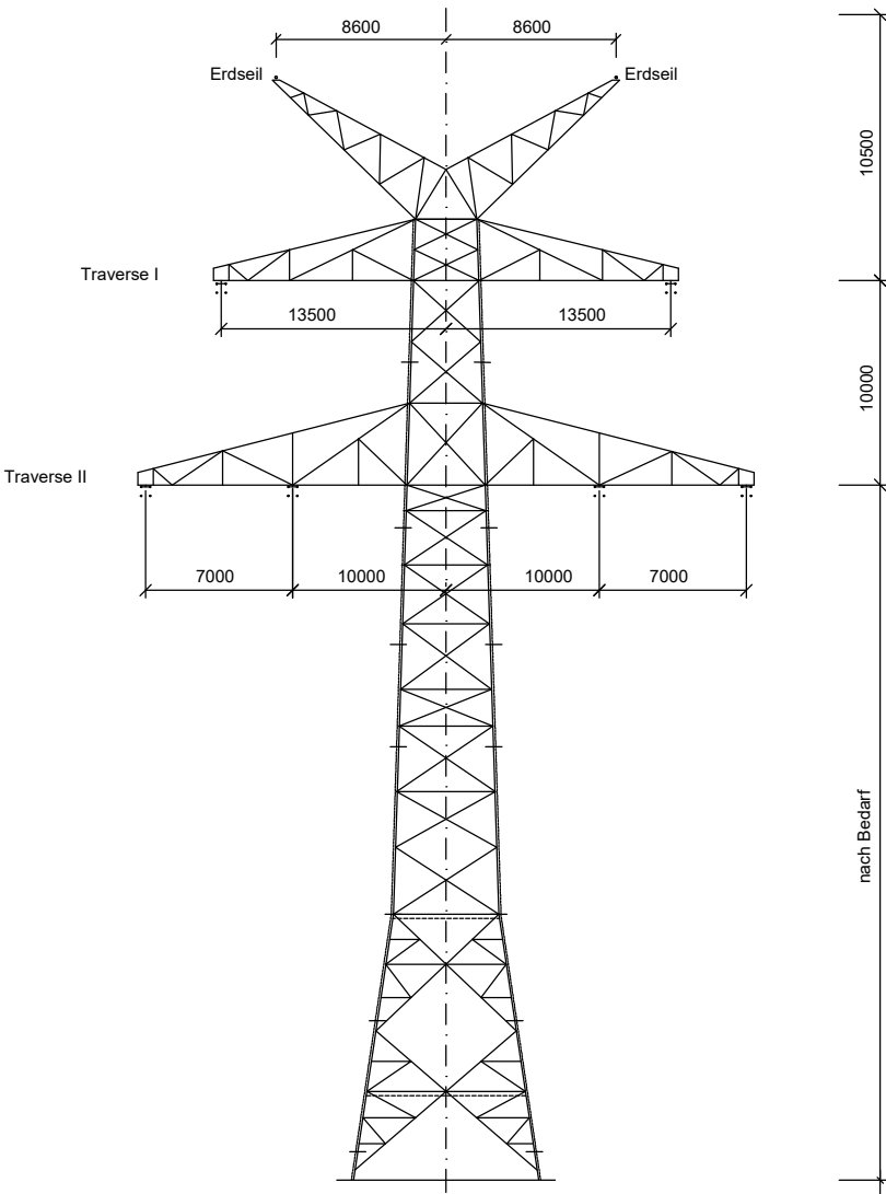
Winkelabspannmast WA120; D-2-D-2018.3 Mast-Nr.: 3, 6, 40, 42, 43, 49
