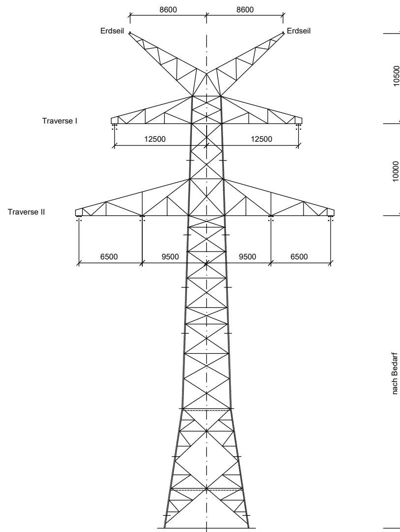
Winkelabspannmast WE/WAdiff140; D-2-D-2018.3 Mast-Nr.: 1, 44, 45
