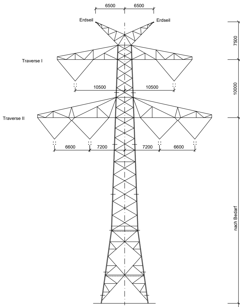
Tragmast T2; D-2-D-2018.3 Mast-Nr.: 20, 38, 39
